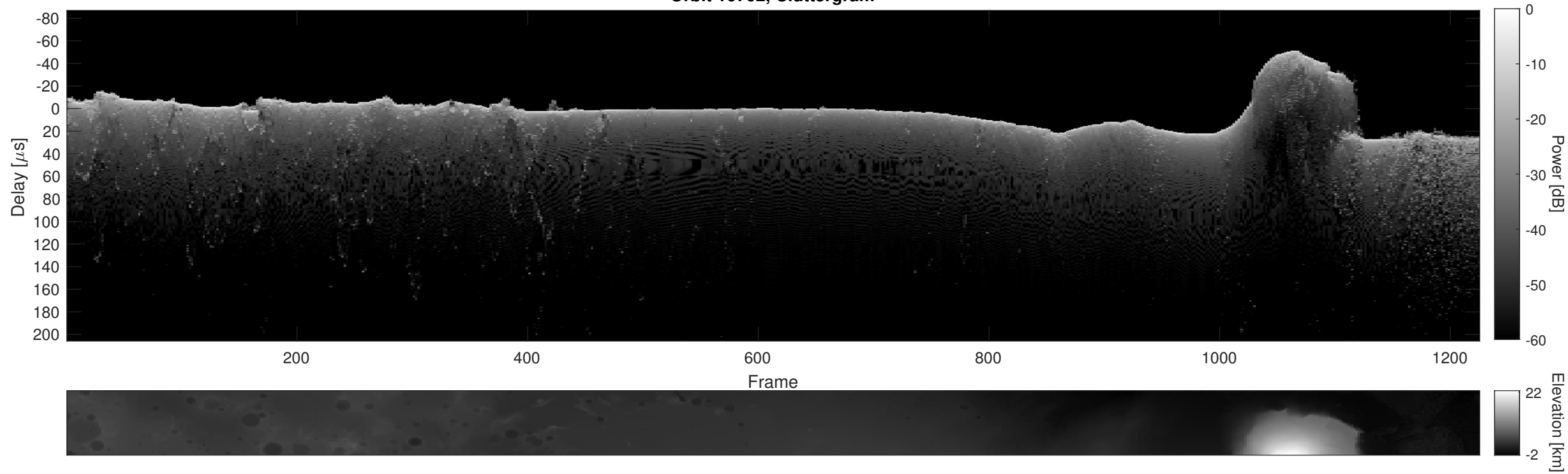
Orbit 16702, Cluttergram
