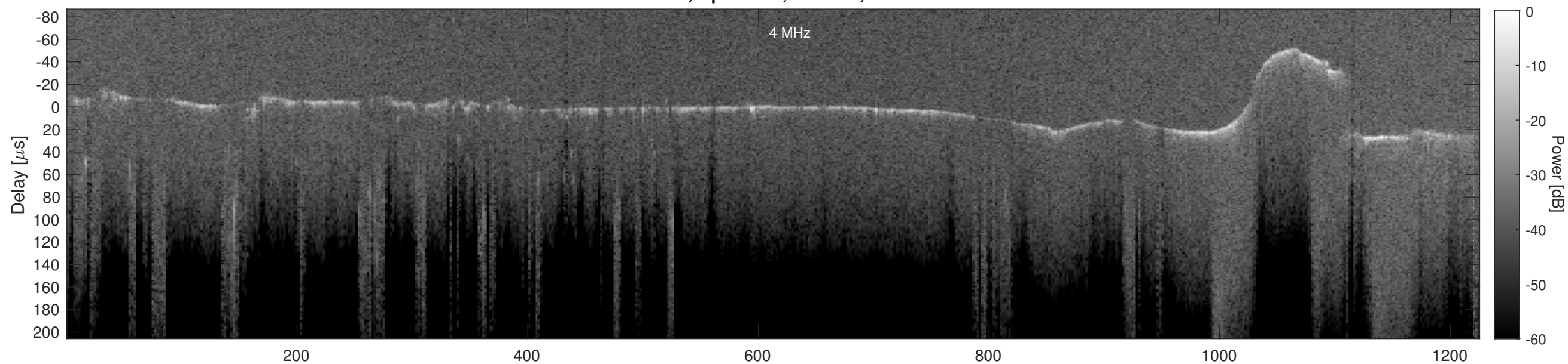
Orbit 16702, Cluttergram
