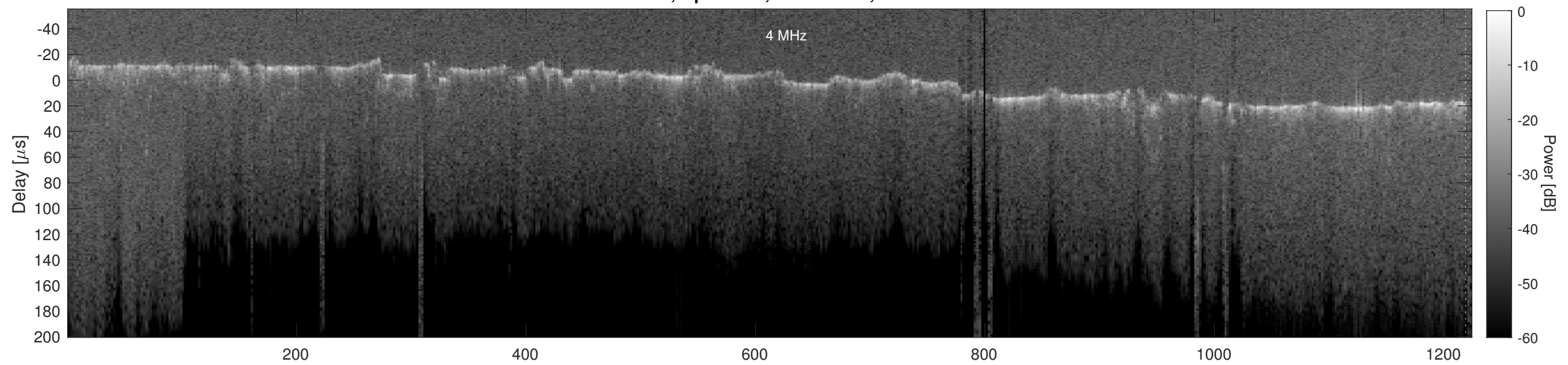
Orbit 16704, Cluttergram
