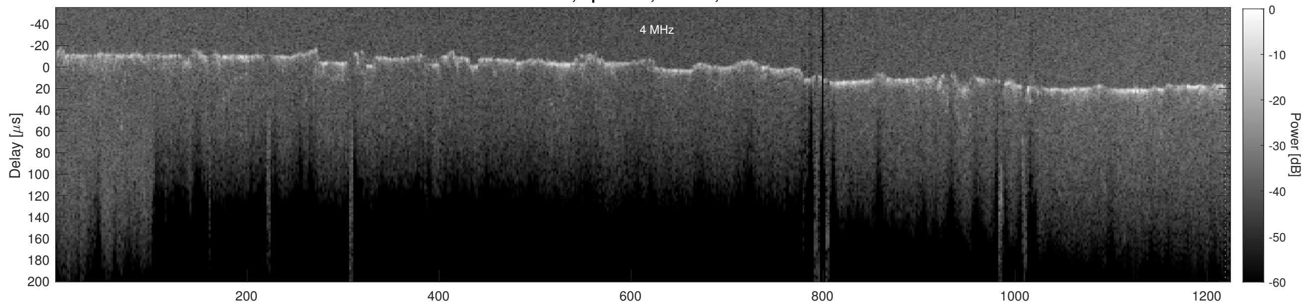
Orbit 16704, Cluttergram
