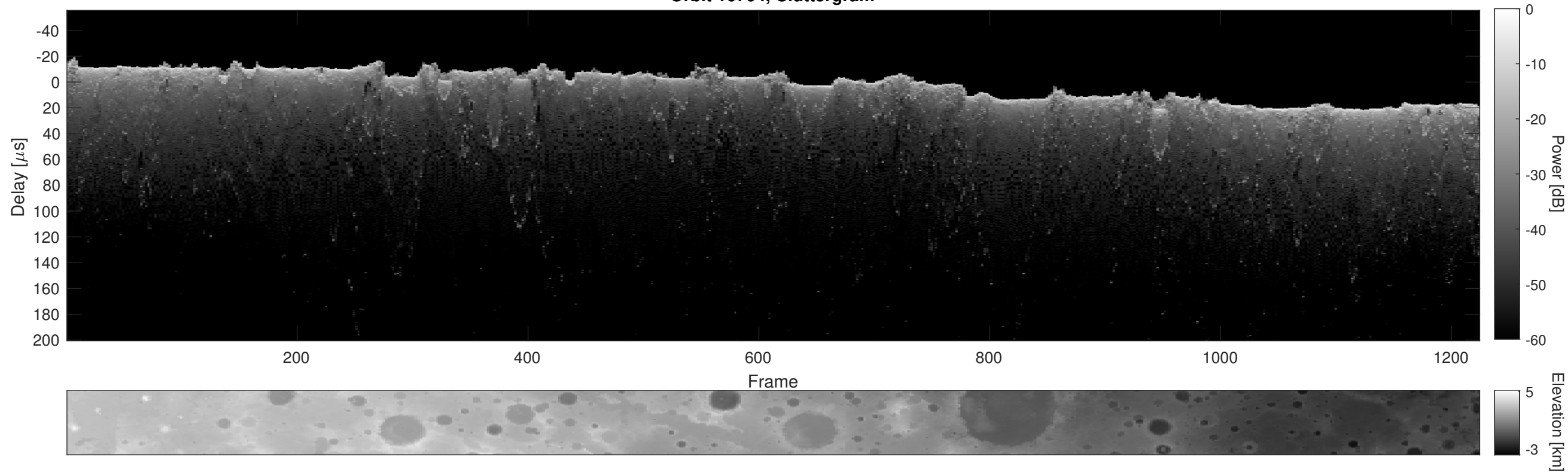
Orbit 16704, Cluttergram
