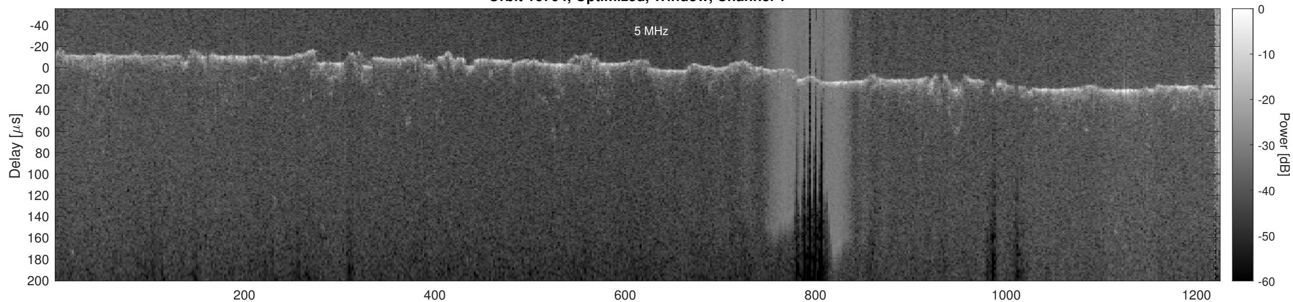
Orbit 16704, Optimized, Window, Channel 2
