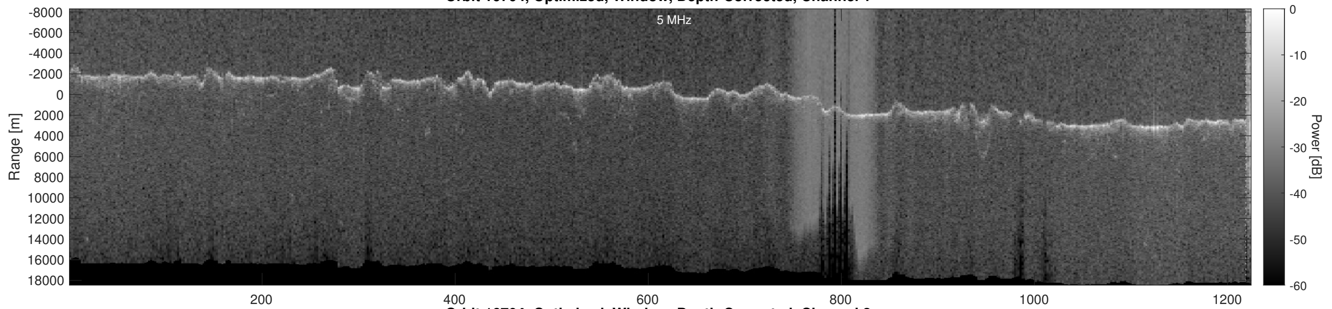
Orbit 16704, Optimized, Window, Depth-Corrected, Channel 2
