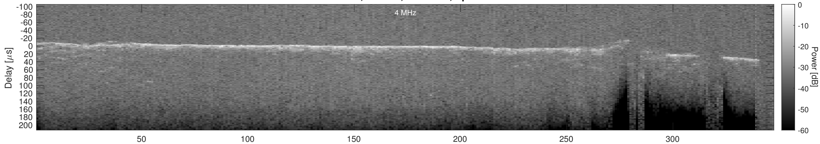
Orbit 16768, Cluttergram
