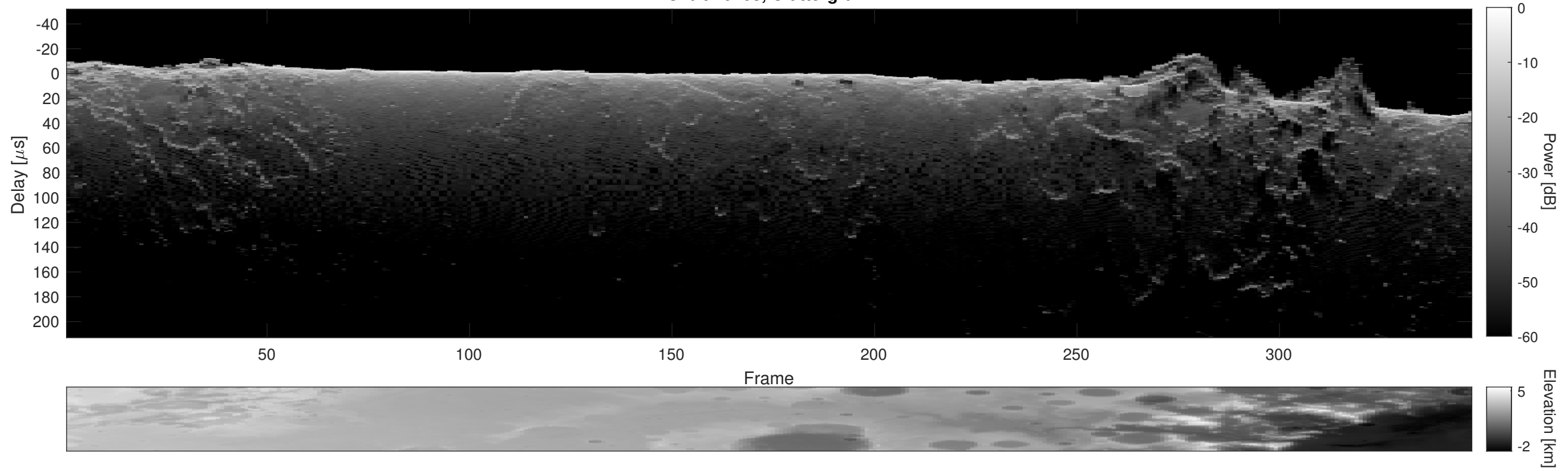
Orbit 16768, Cluttergram
