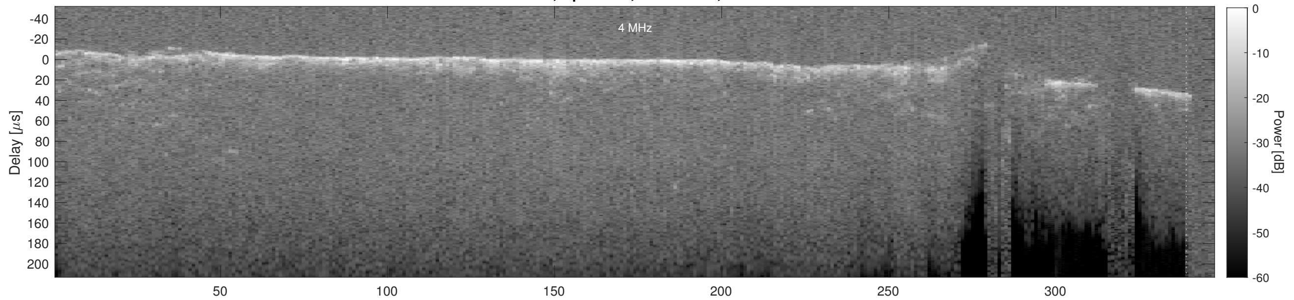
Orbit 16768, Cluttergram
