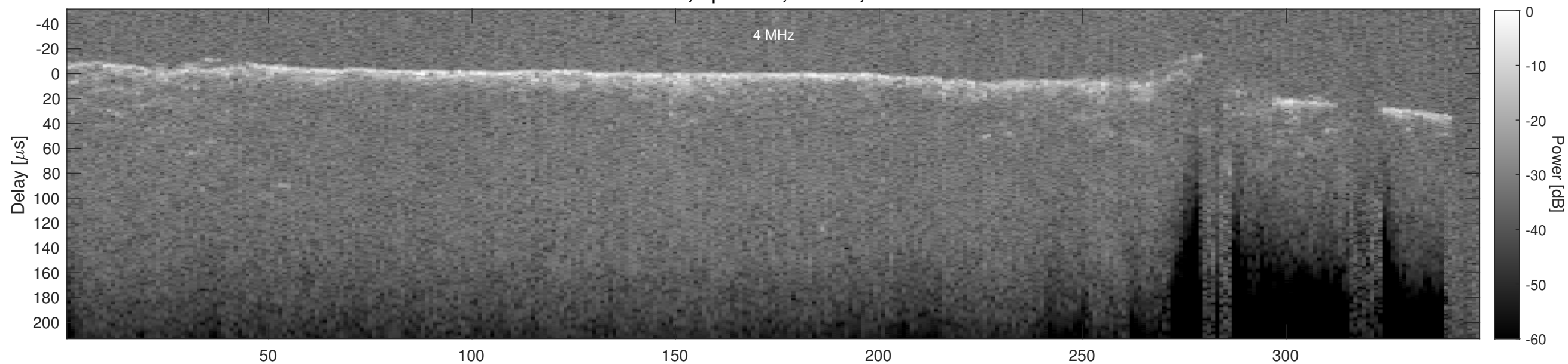
Orbit 16768, Cluttergram
