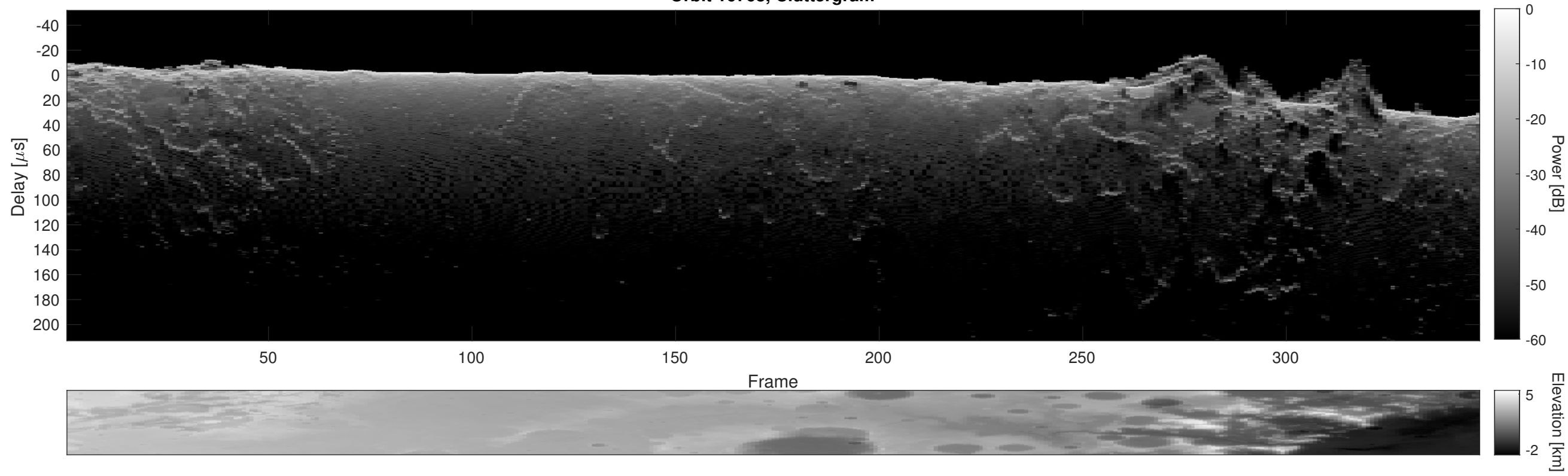
Orbit 16768, Cluttergram
