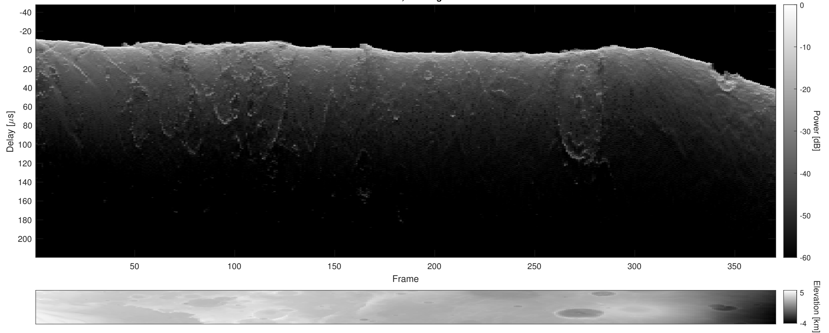
Orbit 16781, Cluttergram
