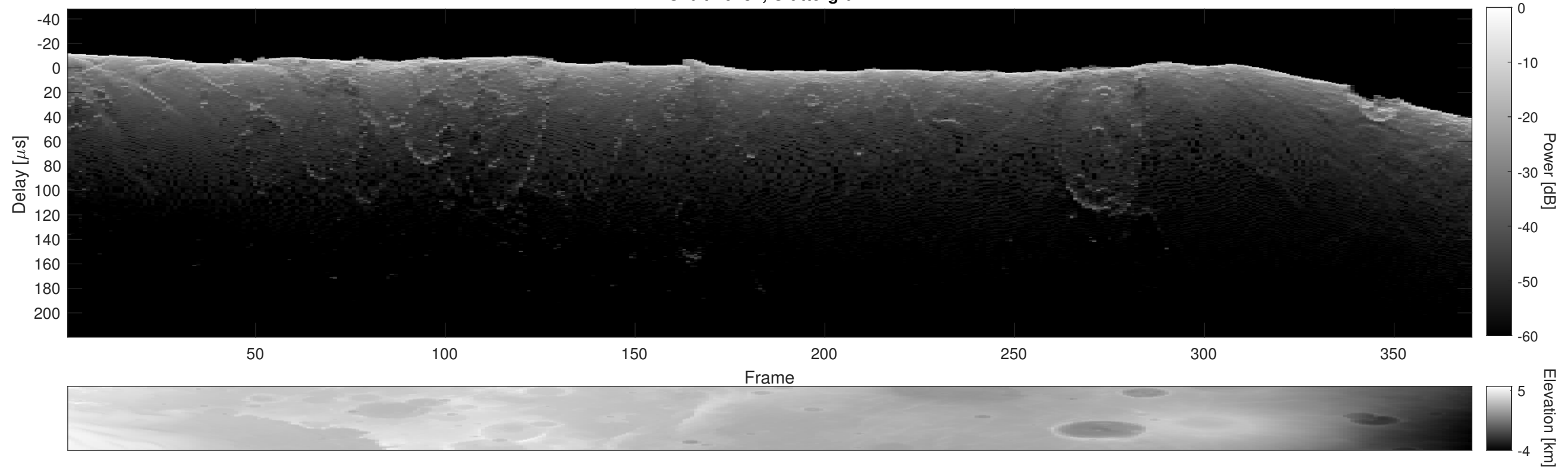
Orbit 16781, Cluttergram
