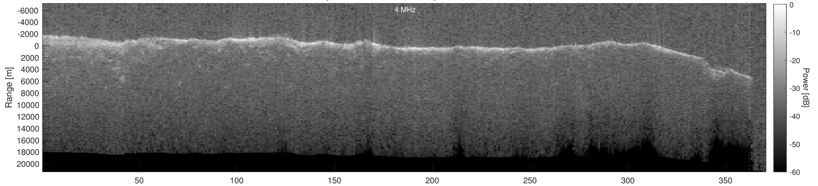
Orbit 16781, Depth-Corrected Cluttergram
