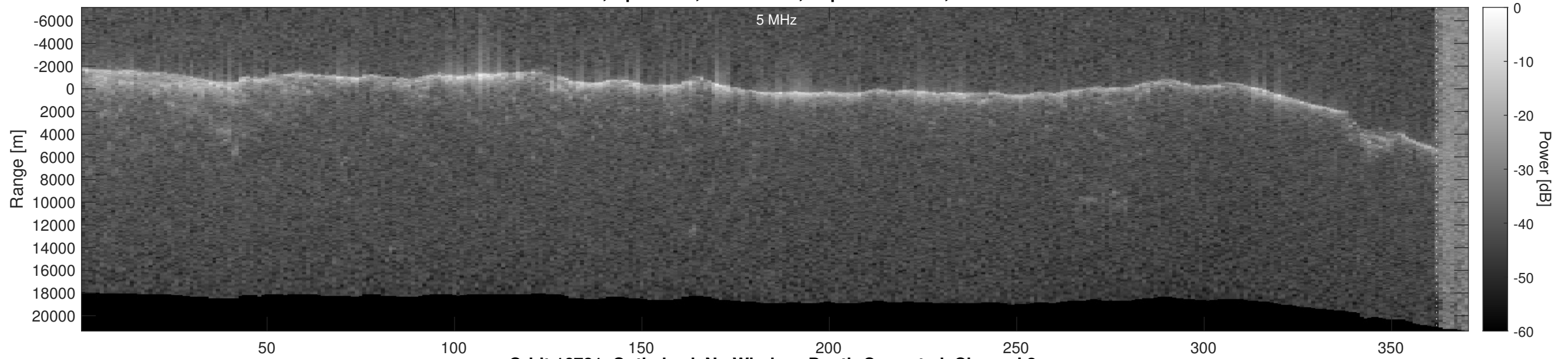
Orbit 16781, Optimized, No Window, Depth-Corrected, Channel 2
