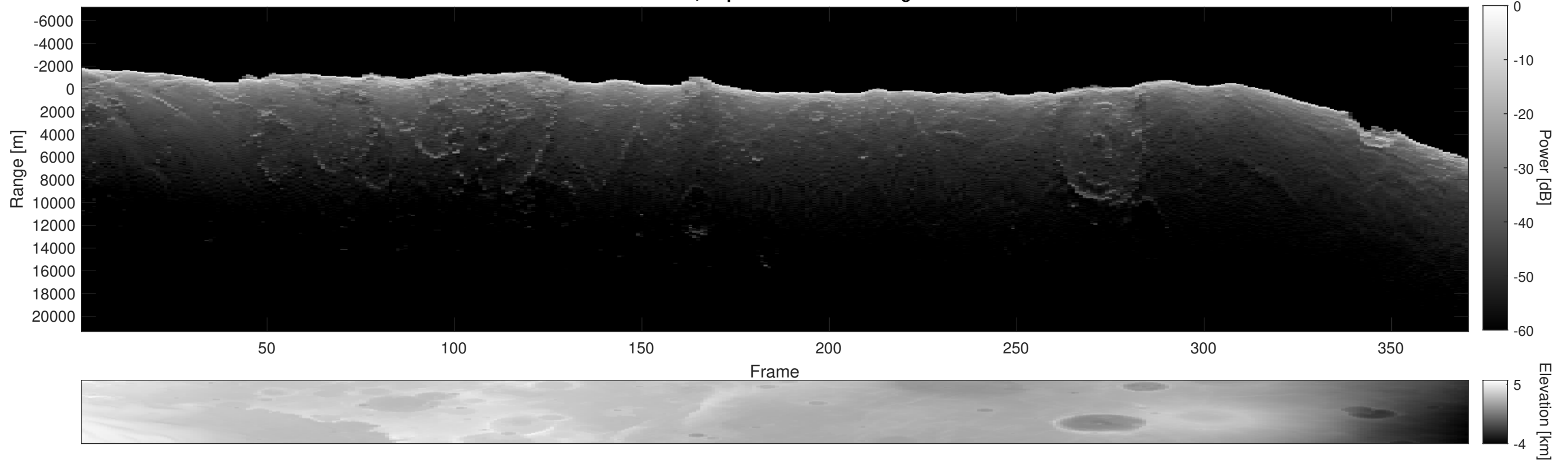
Orbit 16781, Depth-Corrected Cluttergram
