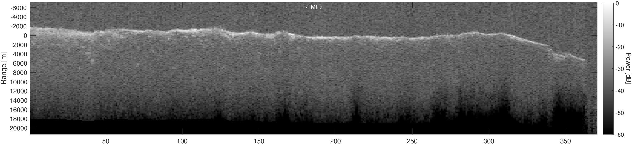
Orbit 16781, Depth-Corrected Cluttergram
