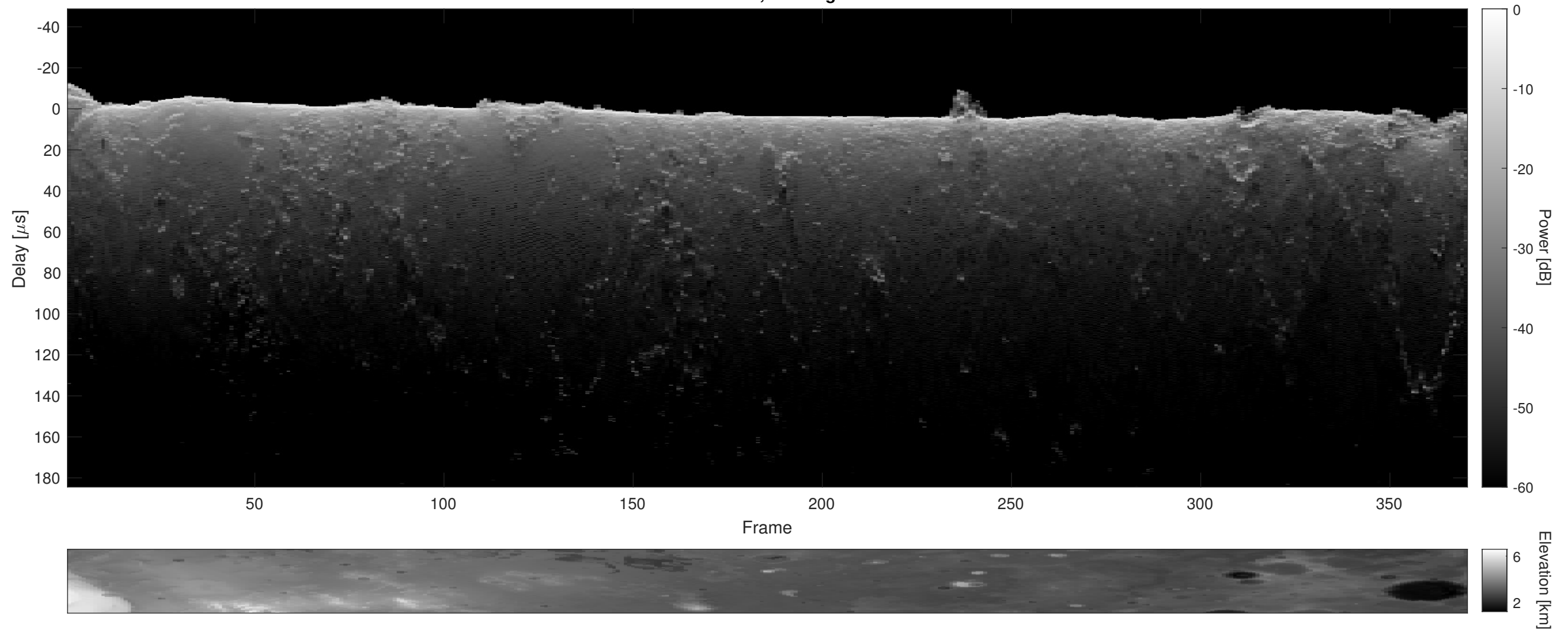
Orbit 16785, Cluttergram
