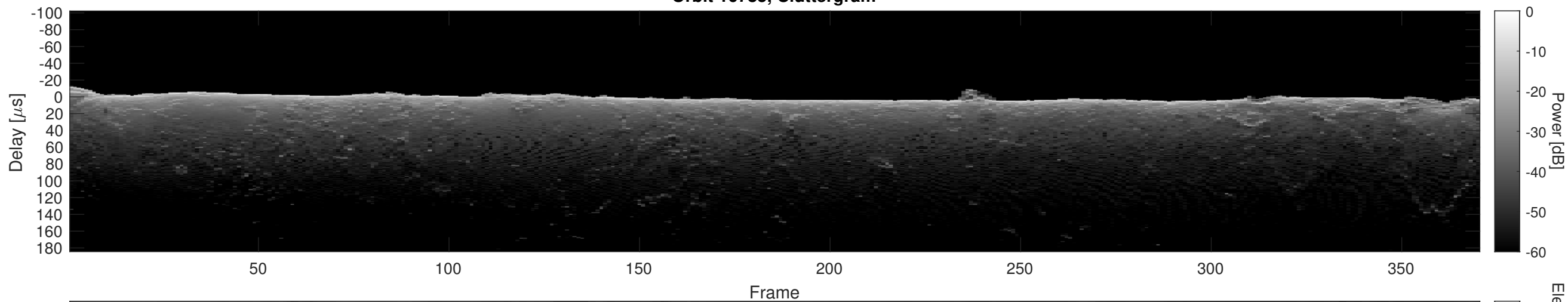
Orbit 16785, Cluttergram
