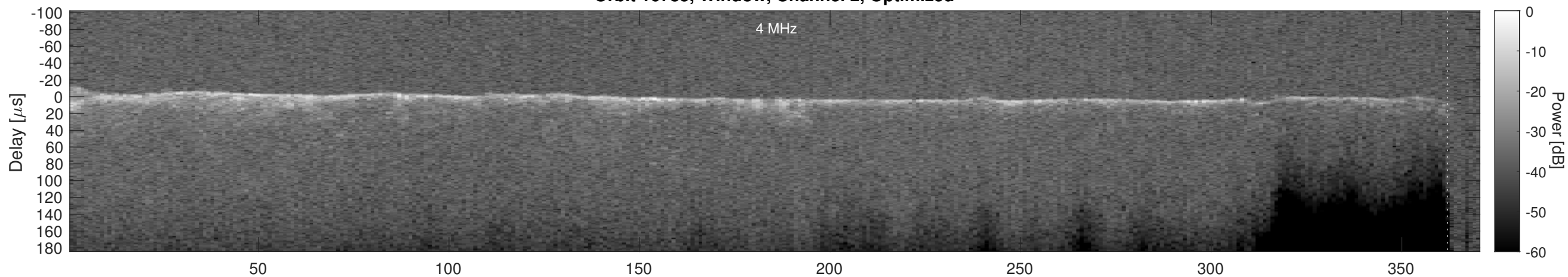
Orbit 16785, Cluttergram
