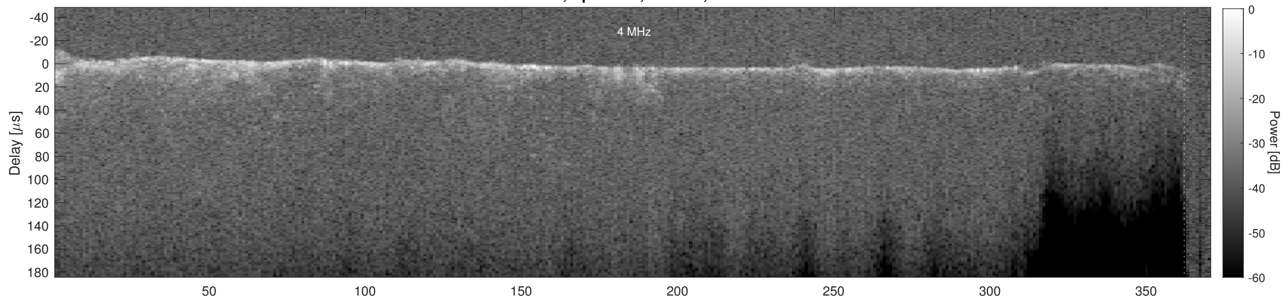
Orbit 16785, Cluttergram
