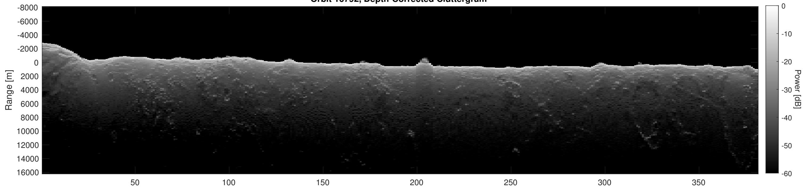
Orbit 16792, Depth-Corrected Cluttergram
