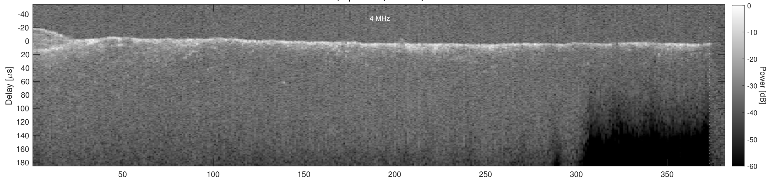
Orbit 16792, Cluttergram
