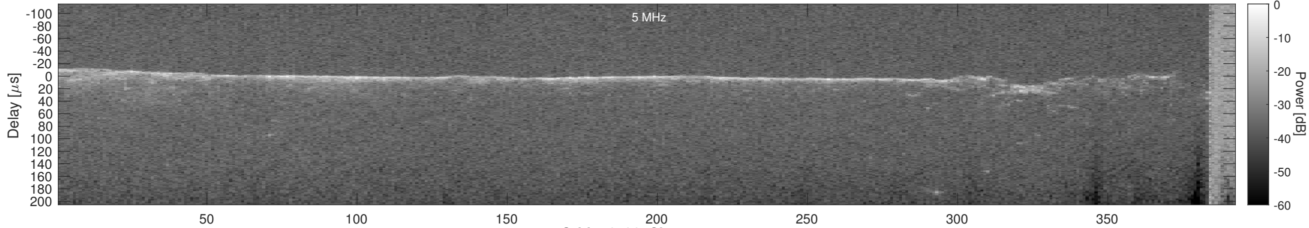
Orbit 16796, Cluttergram
