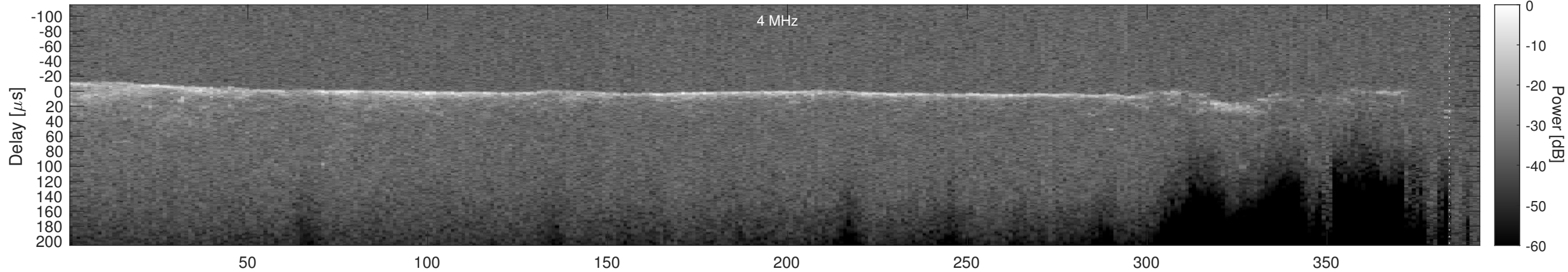
Orbit 16796, Cluttergram
