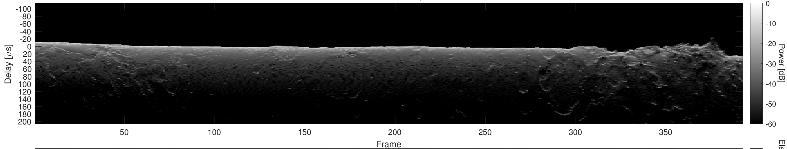
Orbit 16796, Cluttergram
