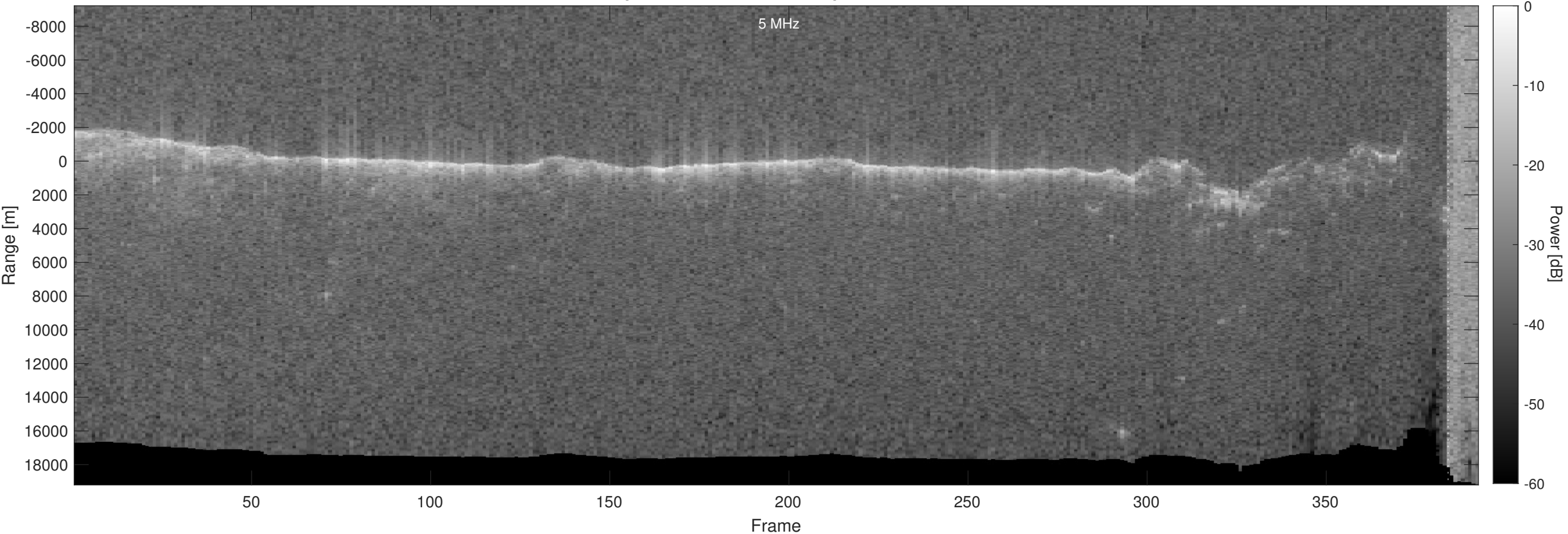
Orbit 16796, Optimized, No Window, Depth-Corrected, Channel 2
