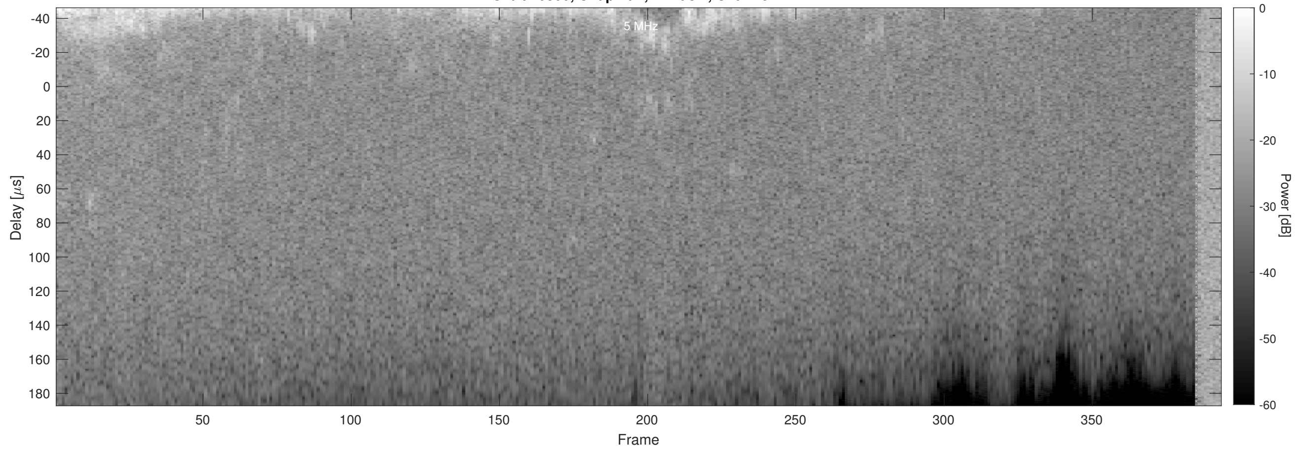
Orbit 16800, Chapman, Window, Channel 2
