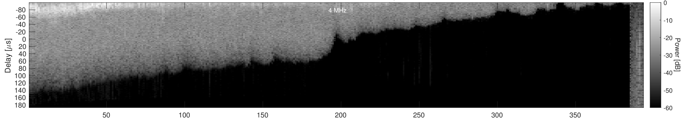
Orbit 16800, Window, Channel 2, Optimized
