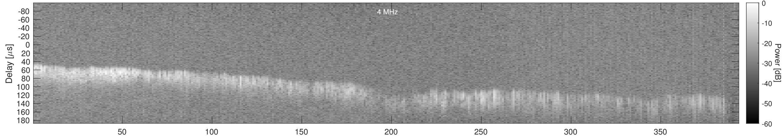
Orbit 16800, Window, Channel 2, Chapman
