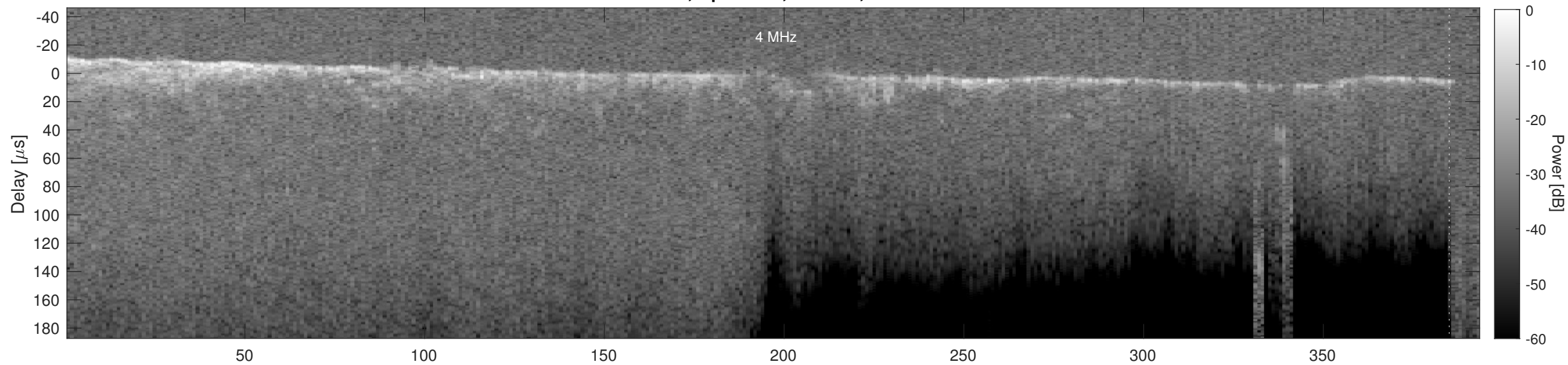
Orbit 16800, Cluttergram
