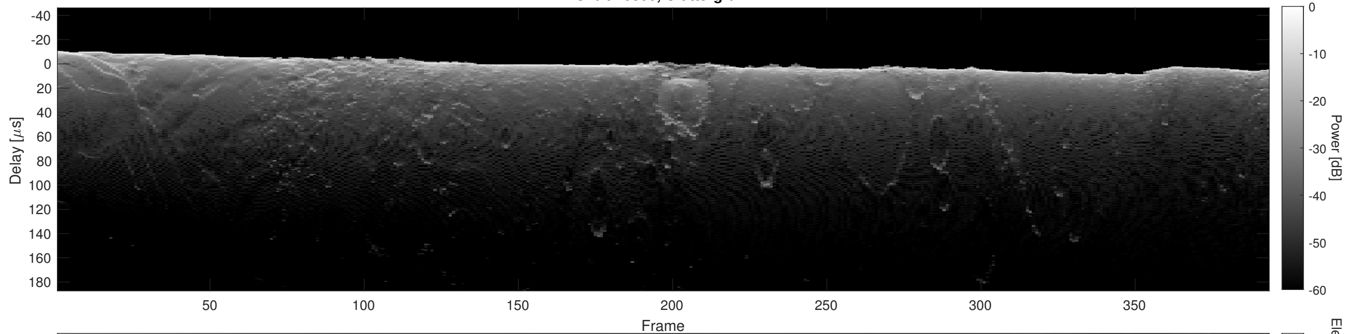
Orbit 16800, Cluttergram
