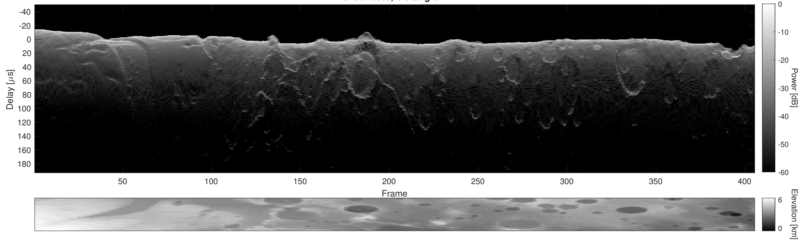
Orbit 16805, Cluttergram
