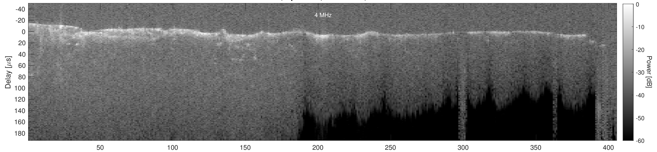
Orbit 16805, Cluttergram
