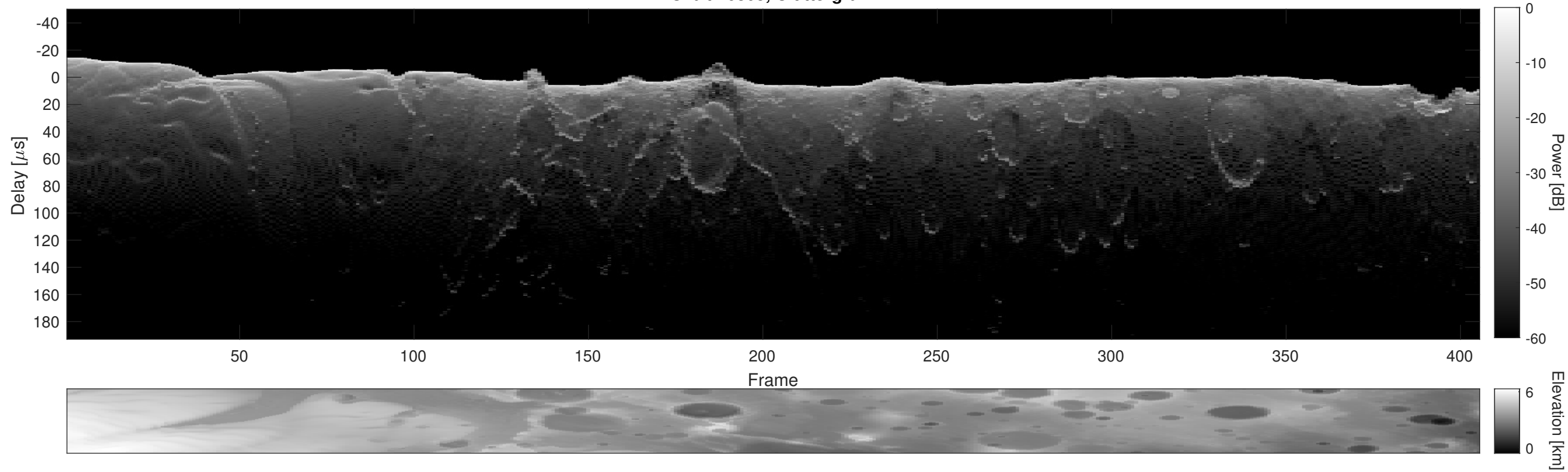
Orbit 16805, Cluttergram
