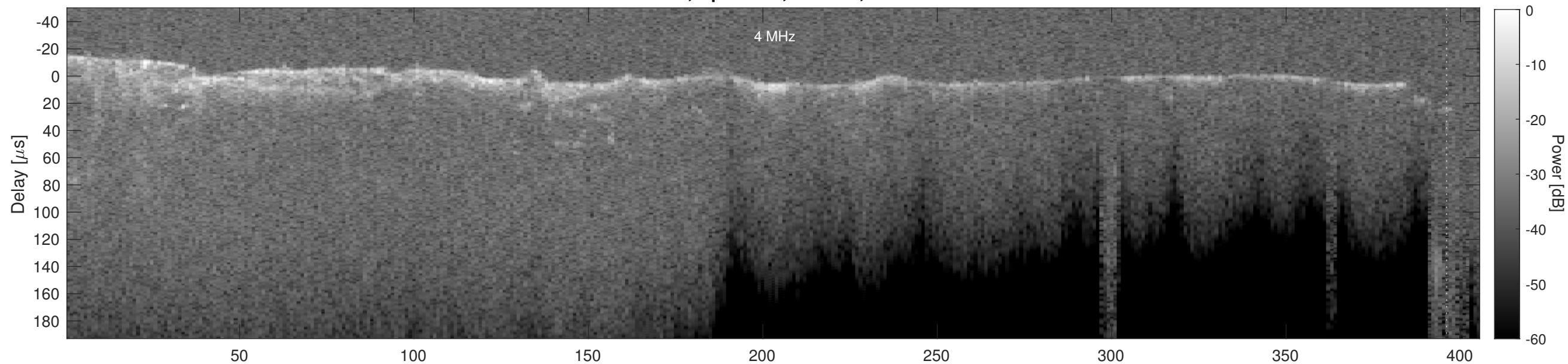
Orbit 16805, Cluttergram
