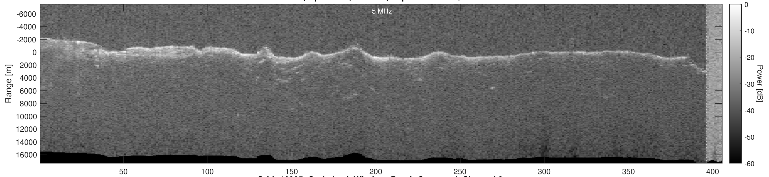
Orbit 16805, Optimized, Window, Depth-Corrected, Channel 2
