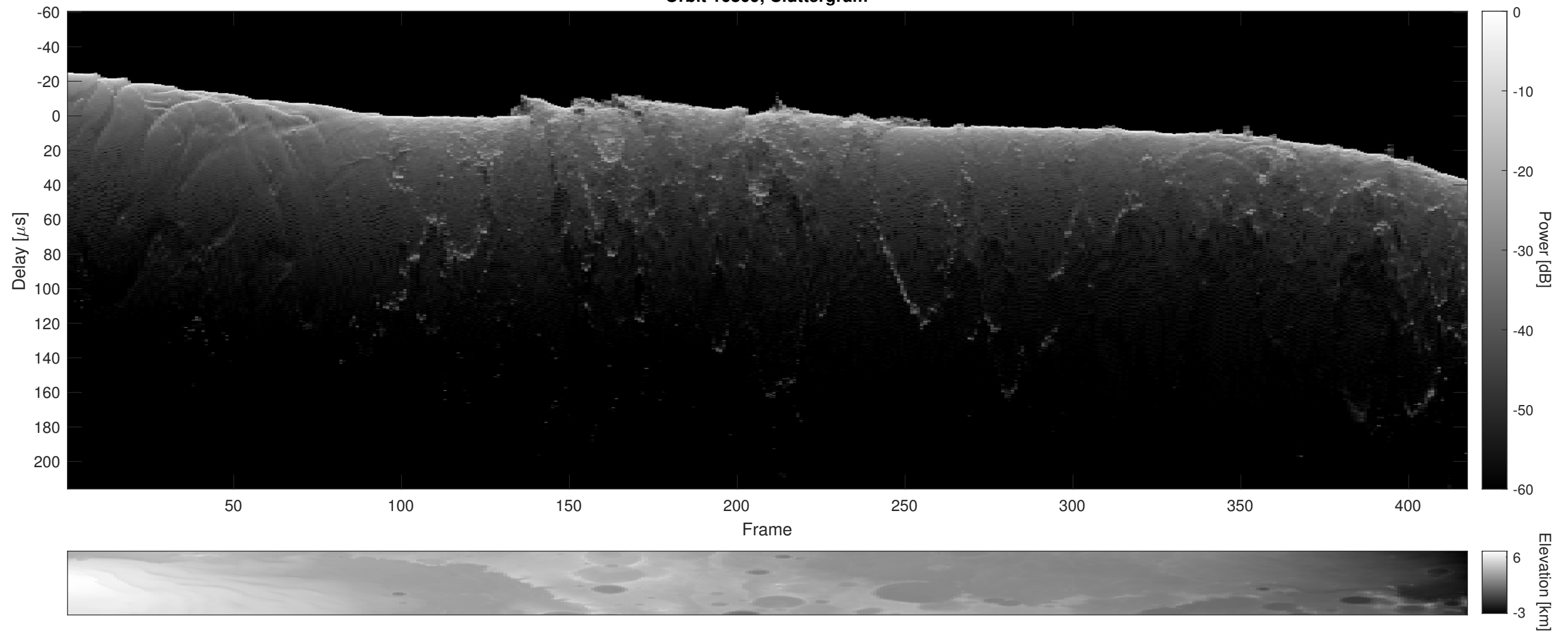
Orbit 16809, Cluttergram
