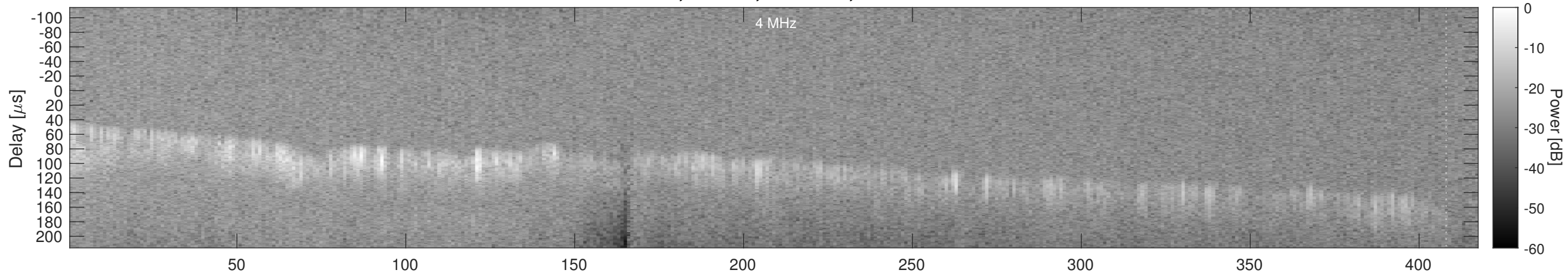
Orbit 16809, Window, Channel 2, Chapman
