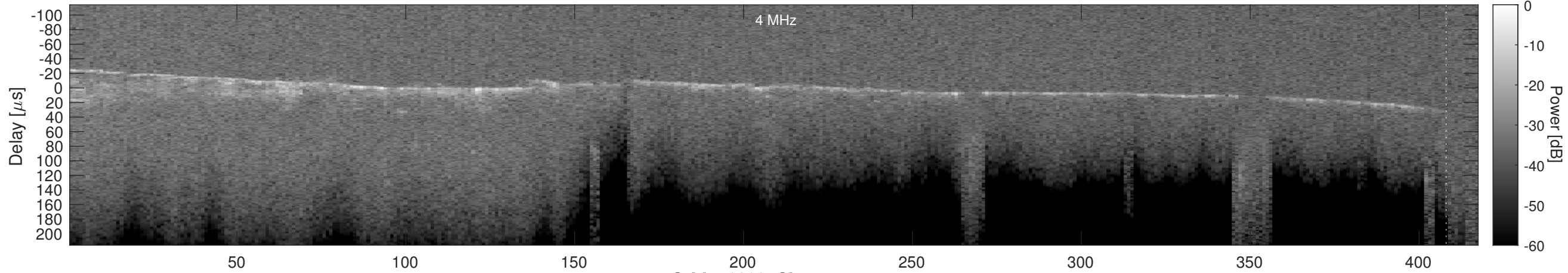
Orbit 16809, Cluttergram
