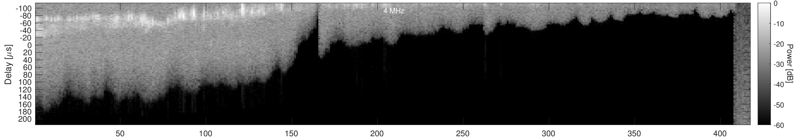
Orbit 16809, Window, Channel 2, Optimized
