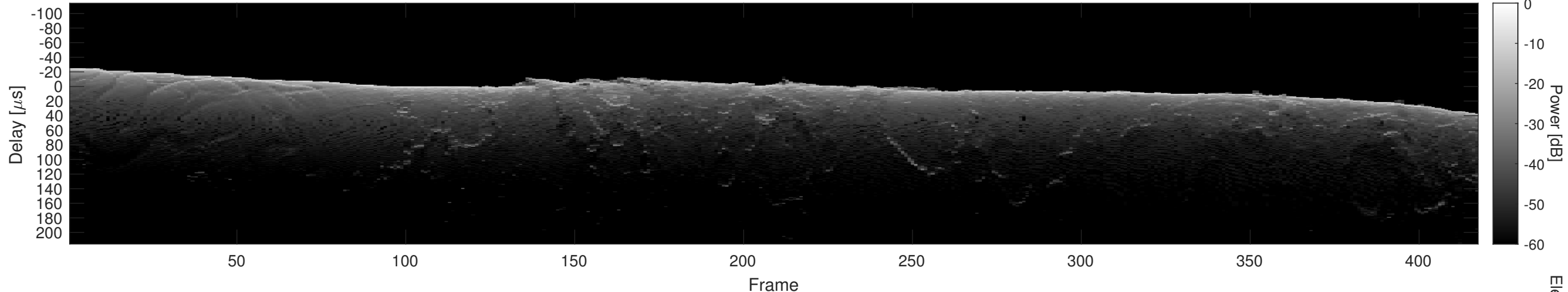
Orbit 16809, Cluttergram
