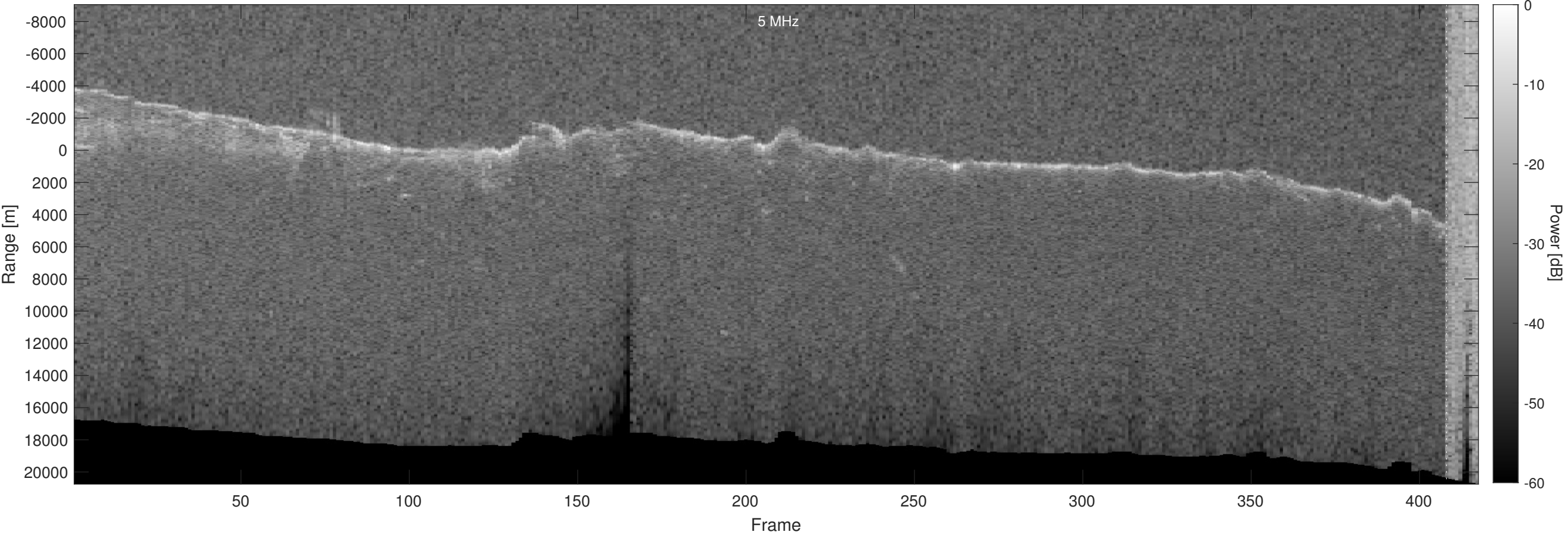
Orbit 16809, Optimized, Window, Depth-Corrected, Channel 2
