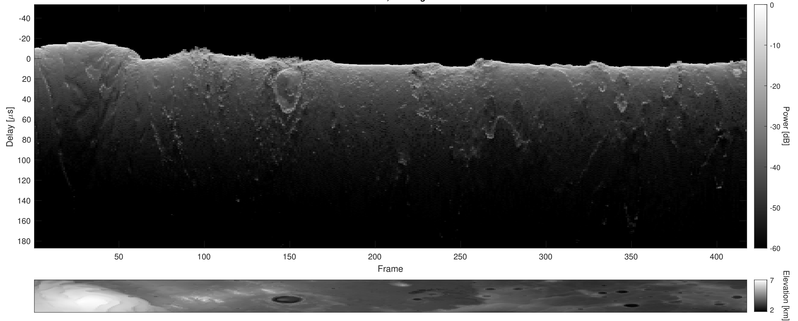
Orbit 16813, Cluttergram
