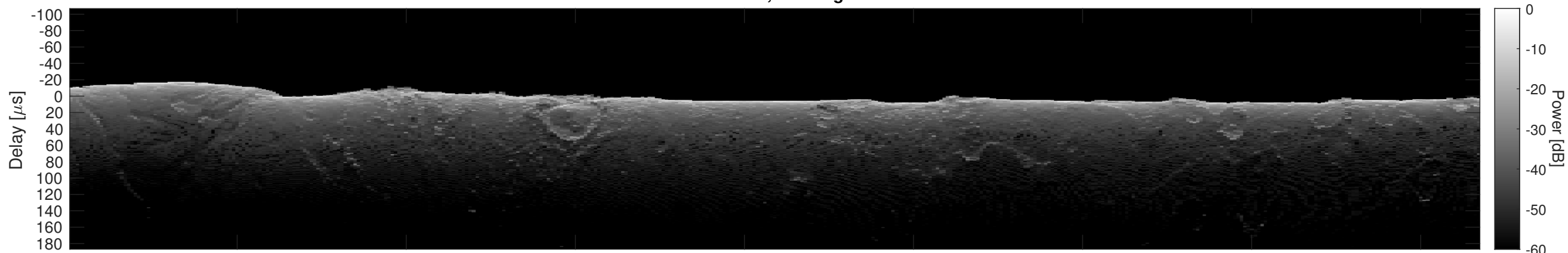
Orbit 16813, Cluttergram
