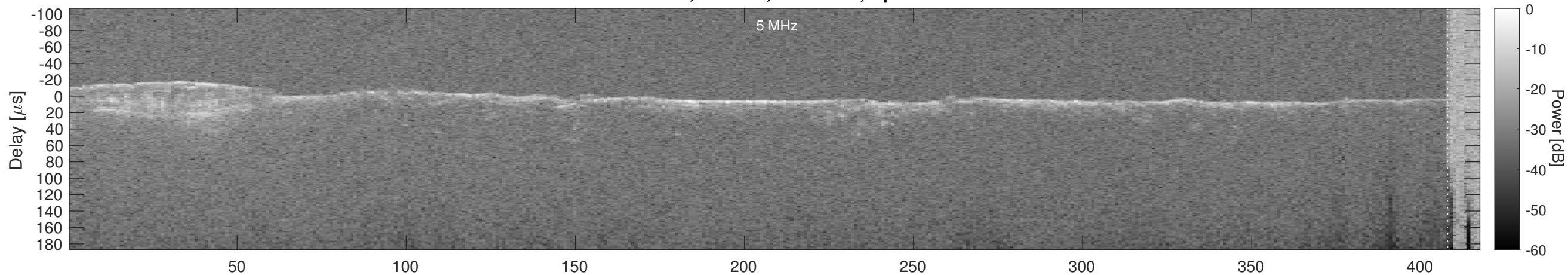
Orbit 16813, Cluttergram
