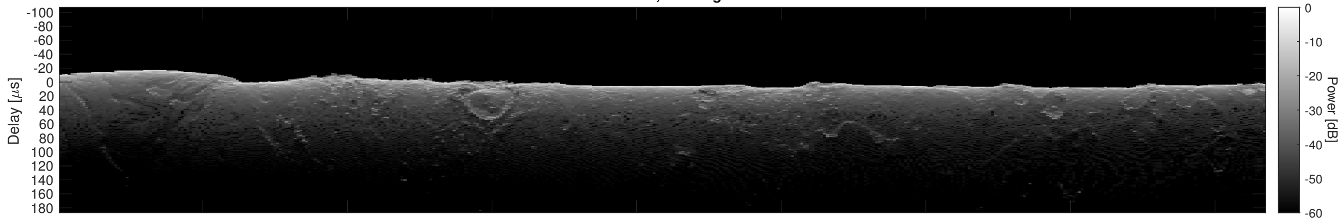
Orbit 16813, Cluttergram
