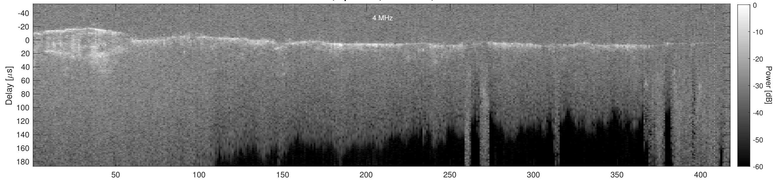
Orbit 16813, Cluttergram
