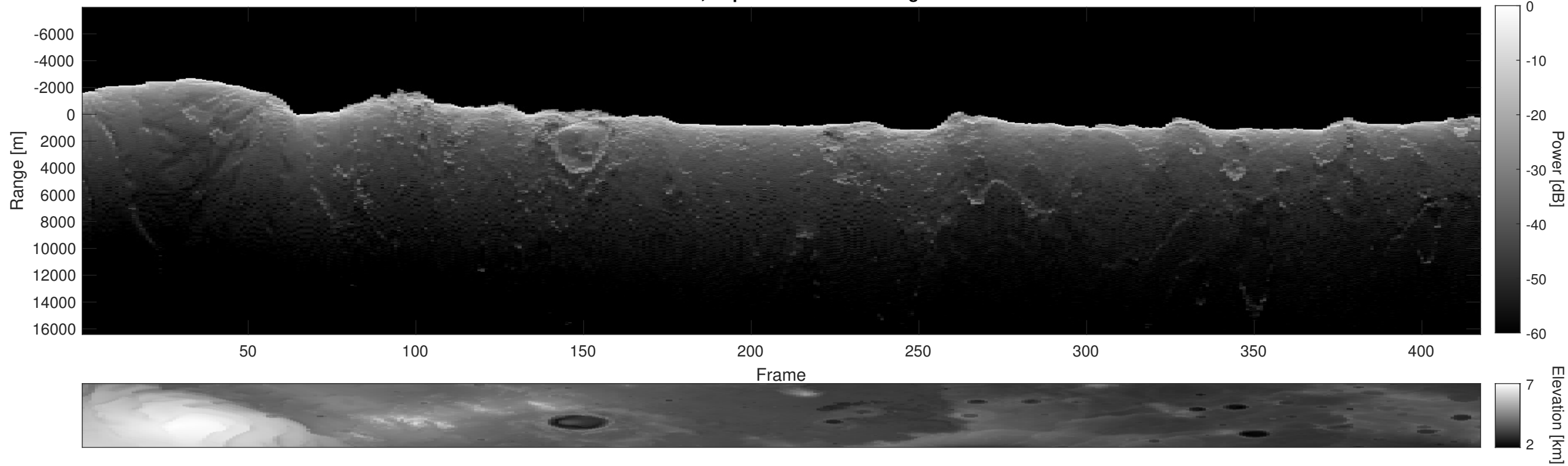
Orbit 16813, Depth-Corrected Cluttergram
