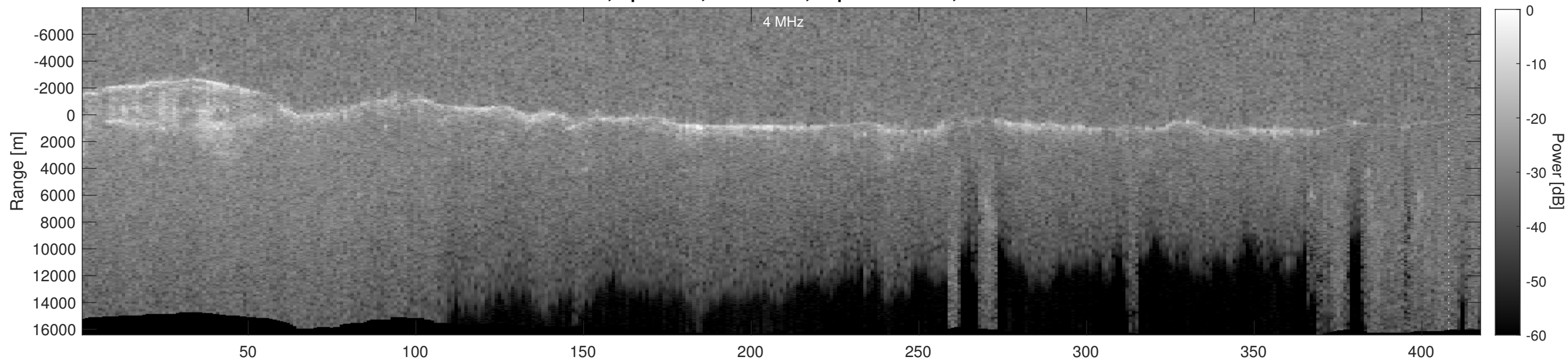
Orbit 16813, Depth-Corrected Cluttergram
