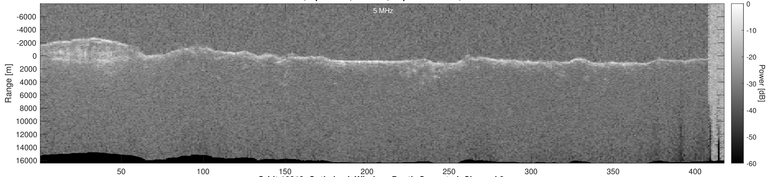
Orbit 16813, Optimized, Window, Depth-Corrected, Channel 2
