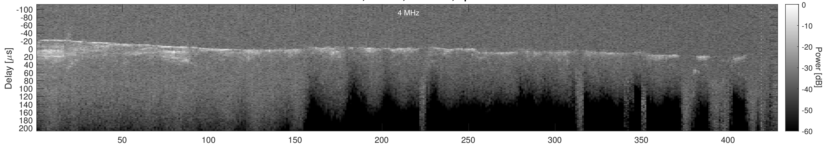
Orbit 16816, Cluttergram
