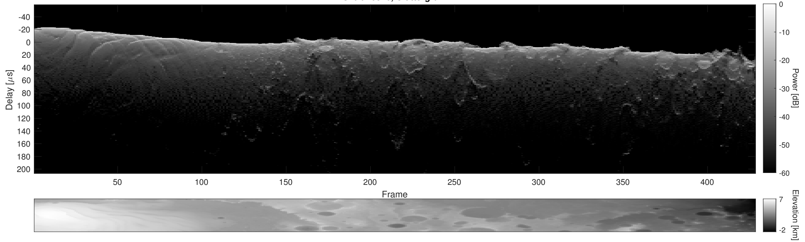
Orbit 16816, Cluttergram
