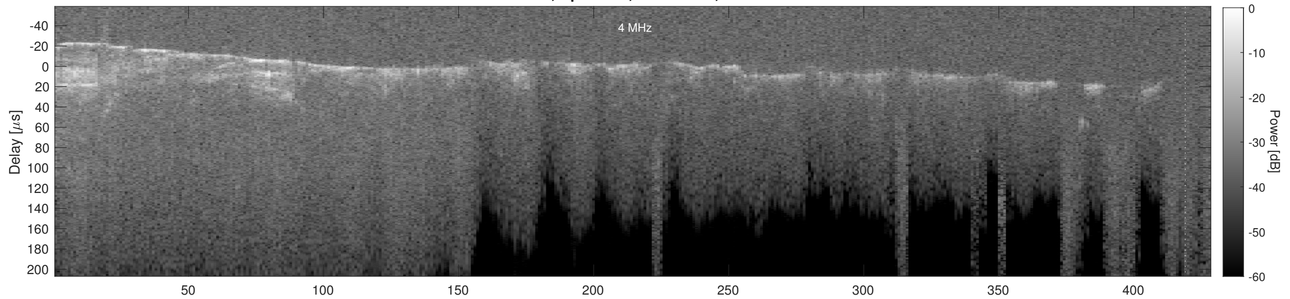
Orbit 16816, Cluttergram
