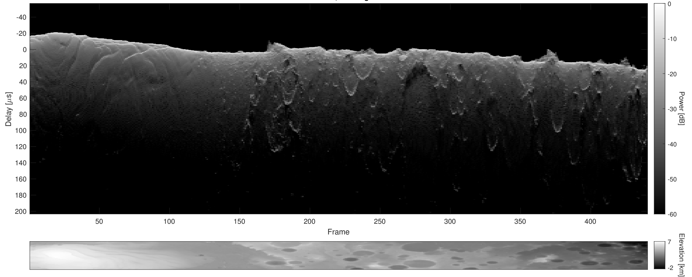
Orbit 16823, Cluttergram
