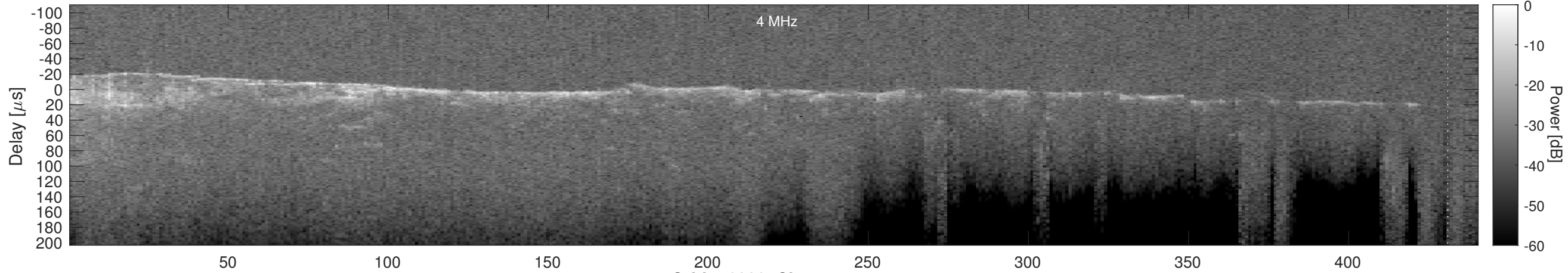
Orbit 16823, Cluttergram
