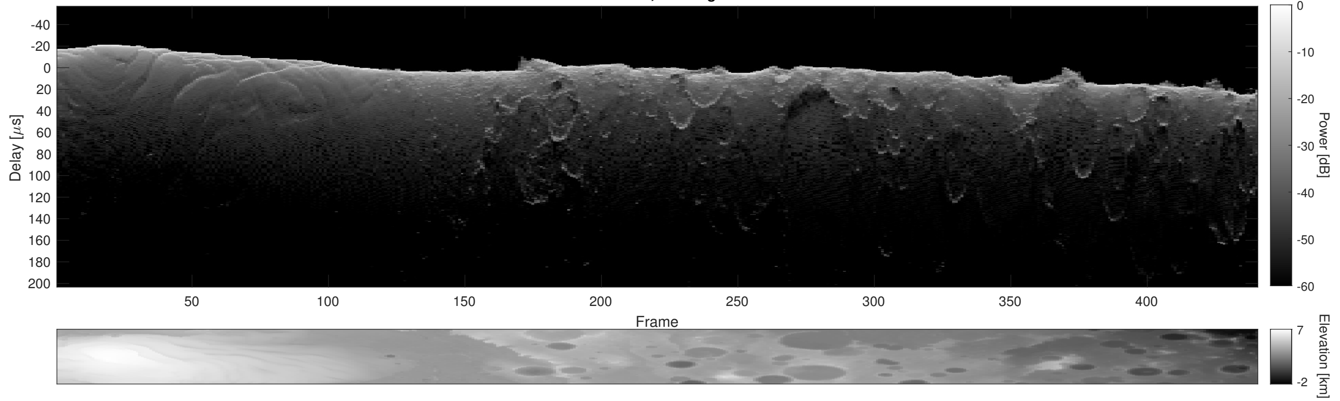
Orbit 16823, Cluttergram
