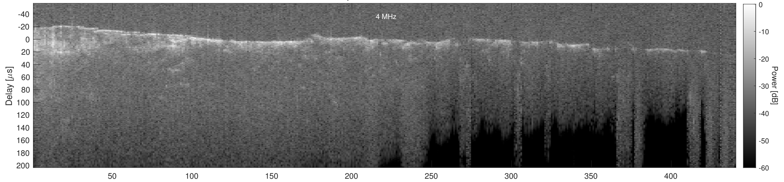
Orbit 16823, Cluttergram
