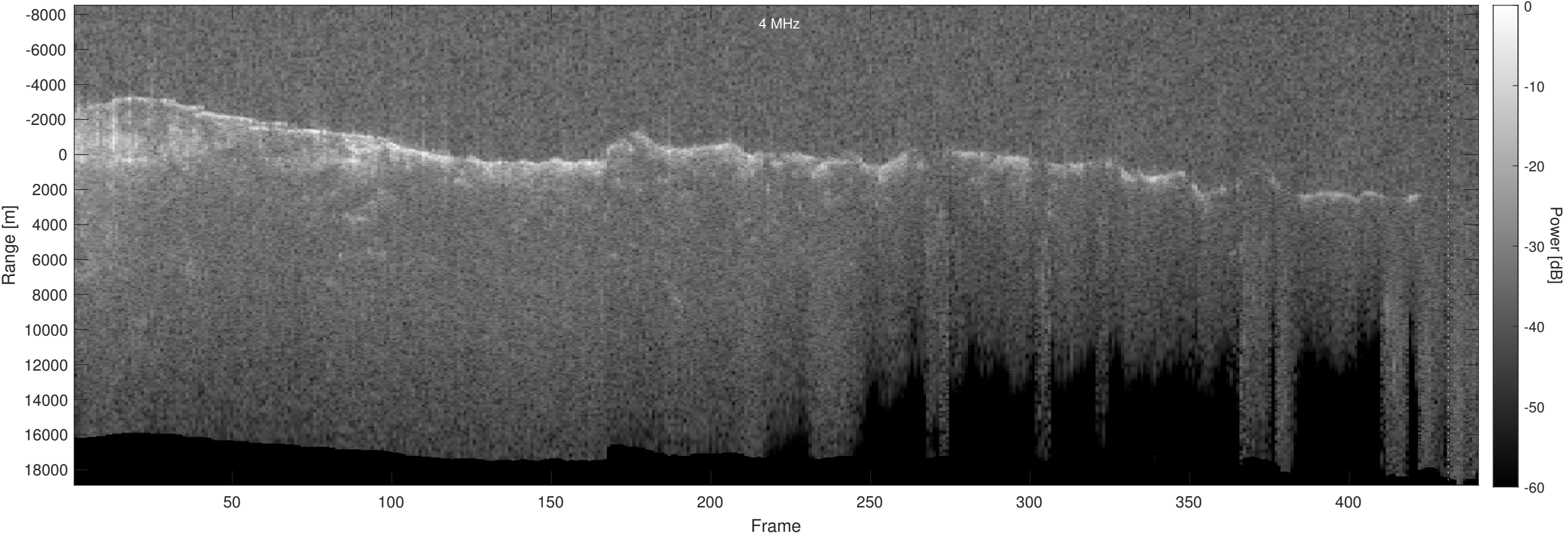
Orbit 16823, Optimized, No Window, Depth-Corrected, Channel 2
