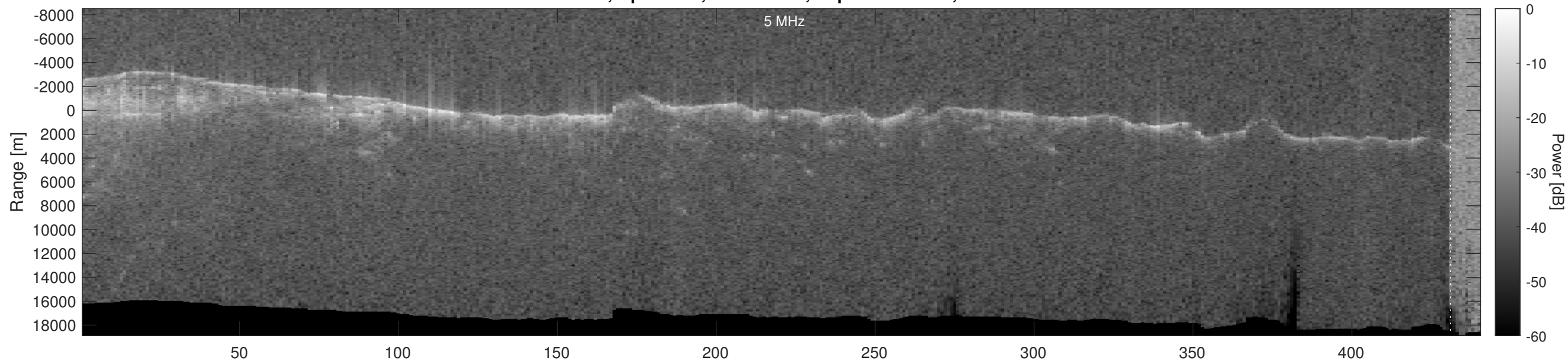
Orbit 16823, Optimized, No Window, Depth-Corrected, Channel 2
