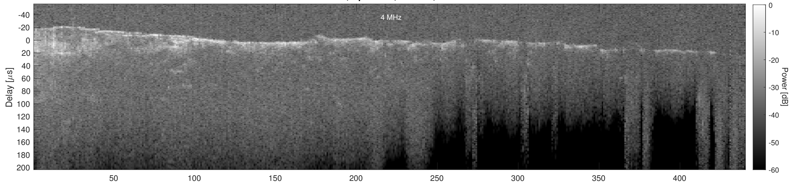
Orbit 16823, Cluttergram
