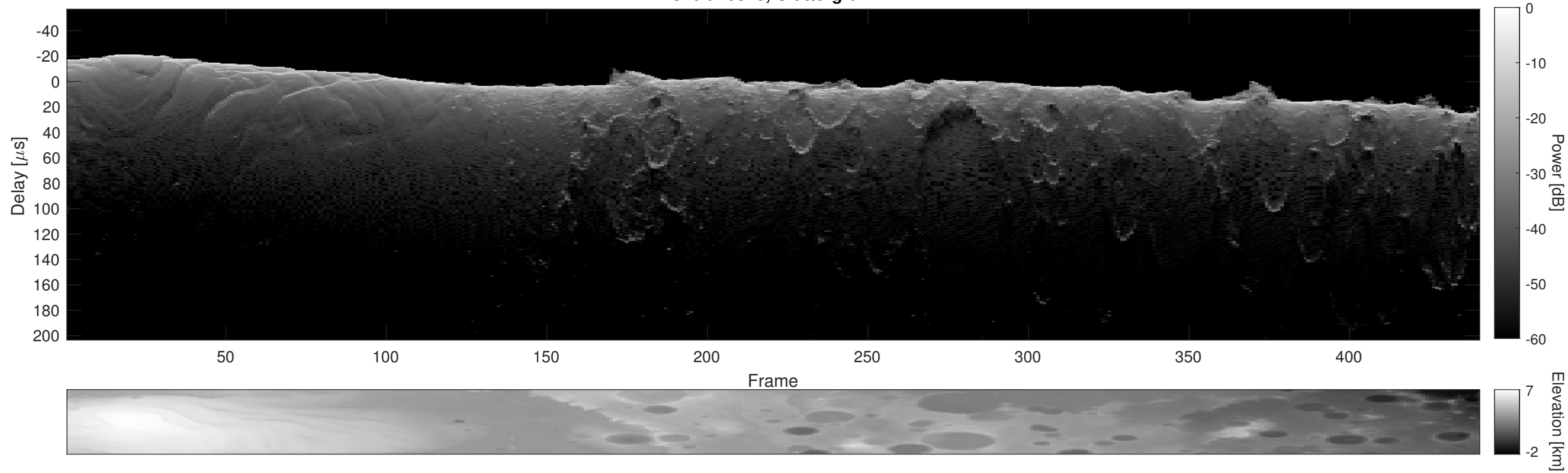
Orbit 16823, Cluttergram
