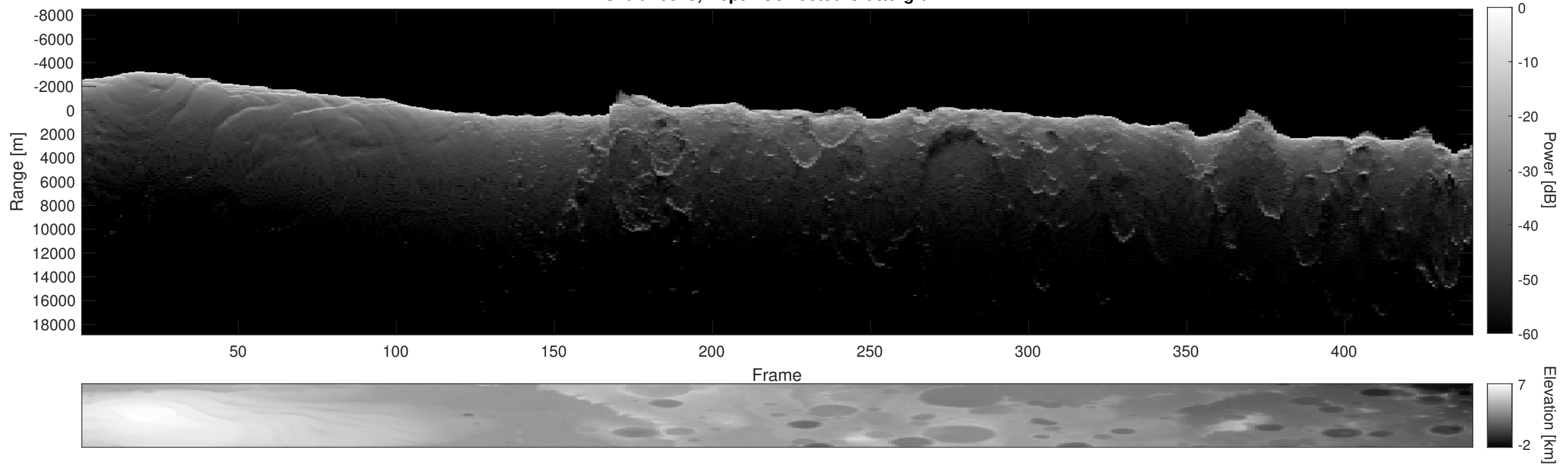
Orbit 16823, Depth-Corrected Cluttergram
