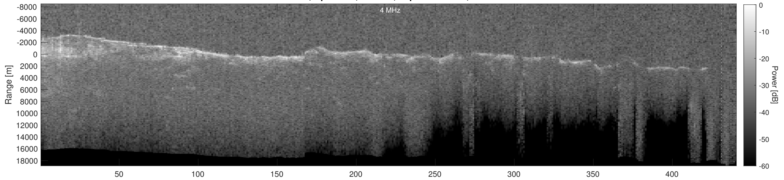
Orbit 16823, Depth-Corrected Cluttergram
