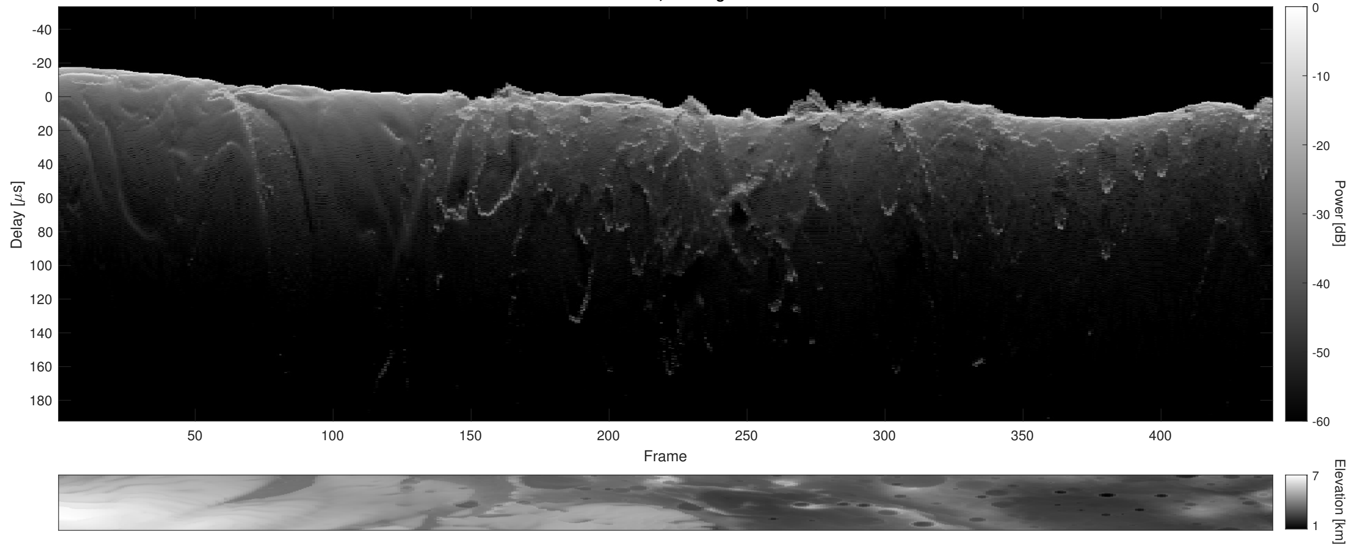
Orbit 16826, Cluttergram
