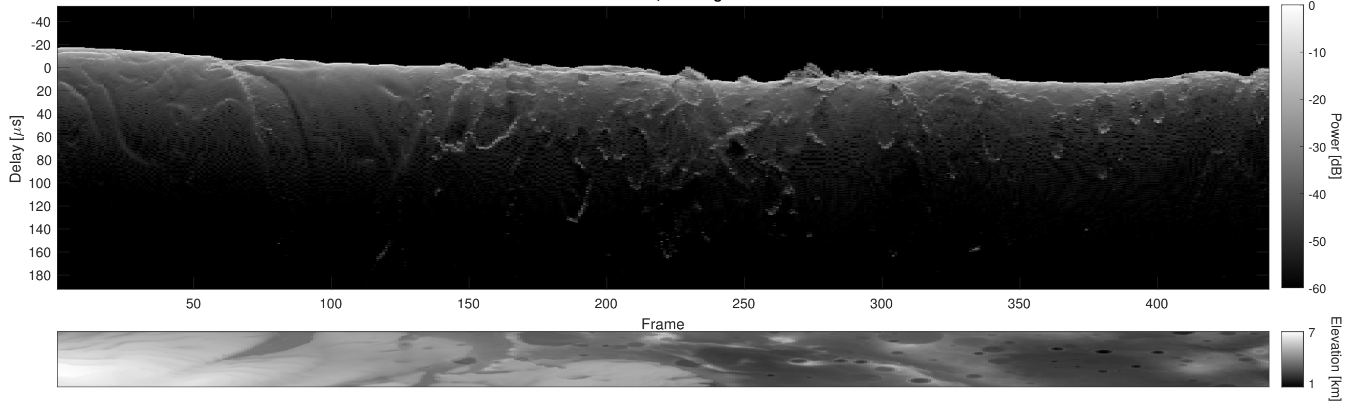
Orbit 16826, Cluttergram
