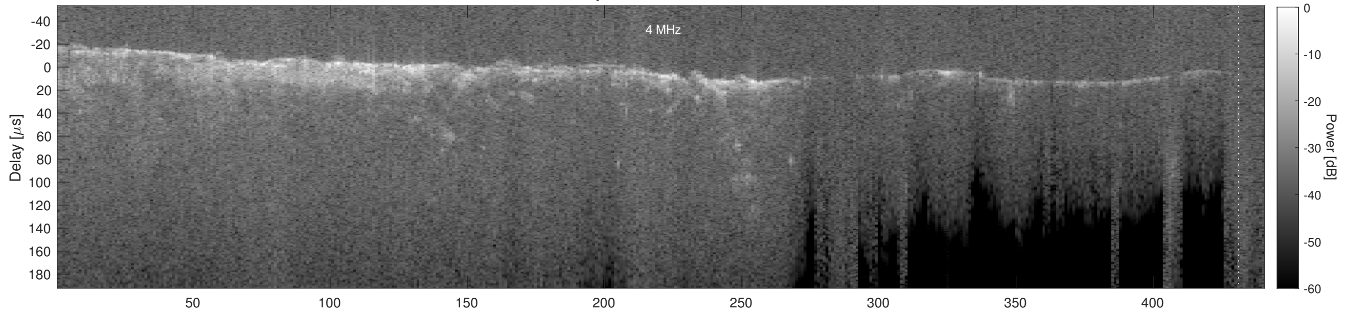
Orbit 16826, Cluttergram
