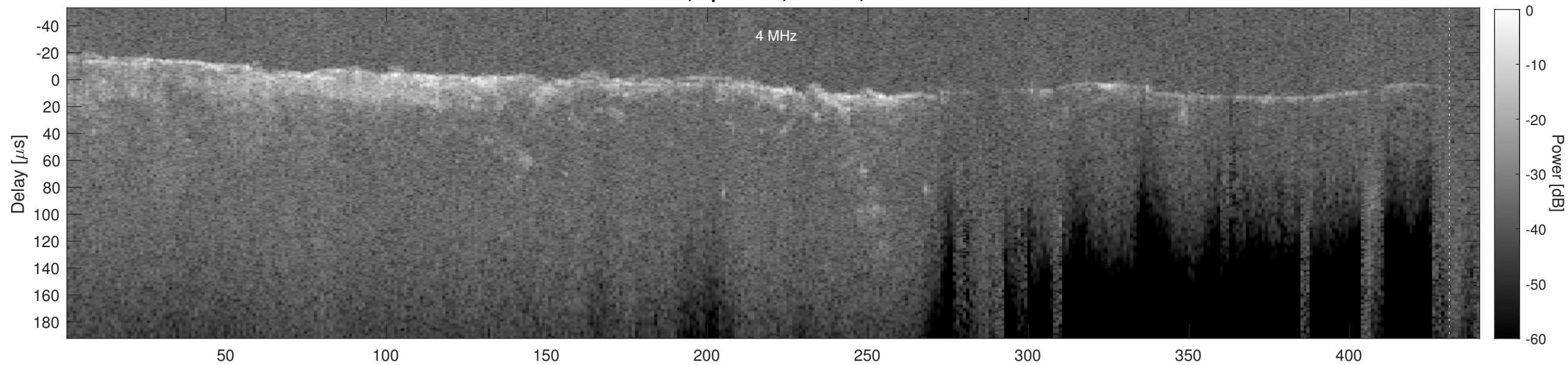
Orbit 16826, Cluttergram
