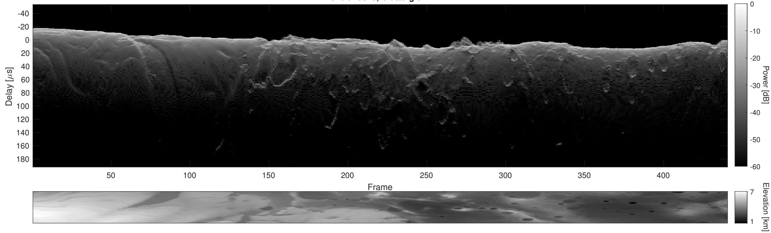
Orbit 16826, Cluttergram
