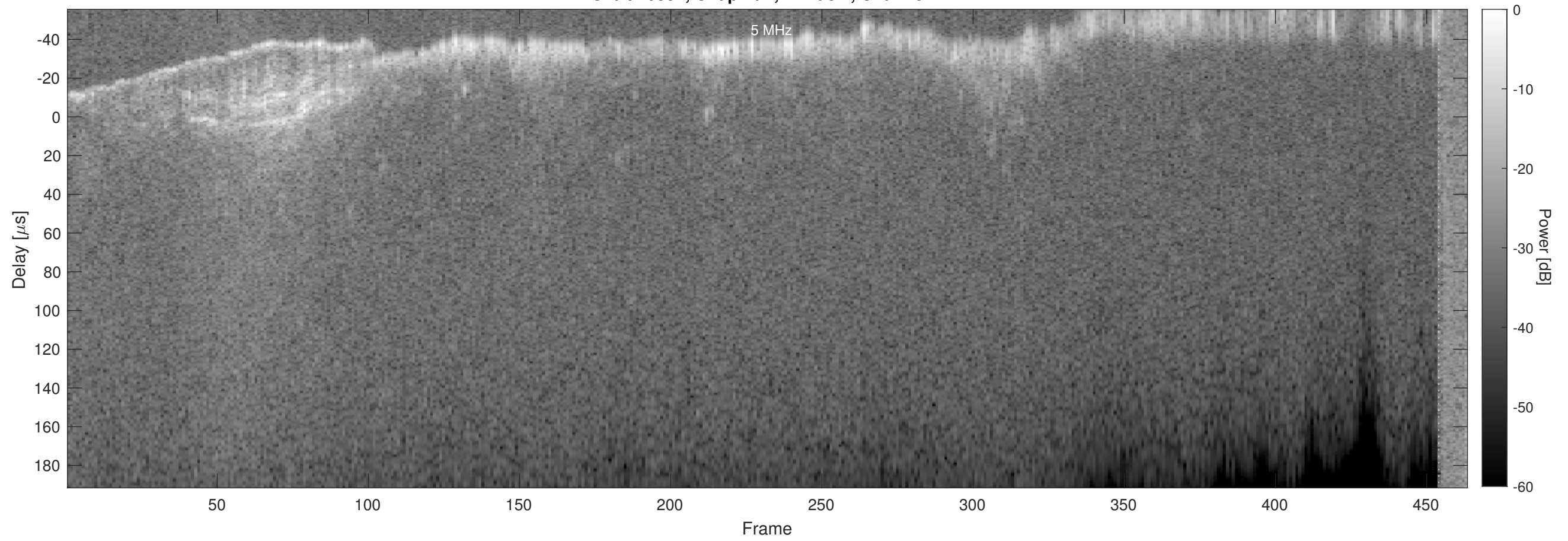
Orbit 16834, Chapman, Window, Channel 2
