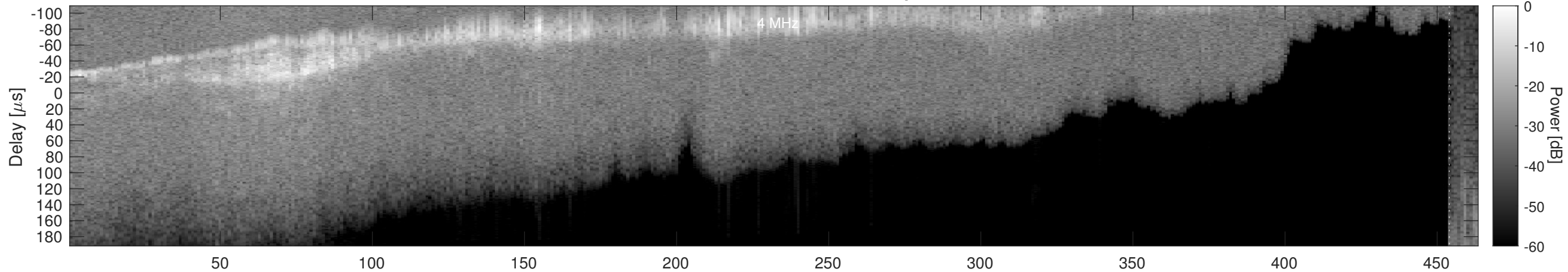
Orbit 16834, Window, Channel 2, Optimized
