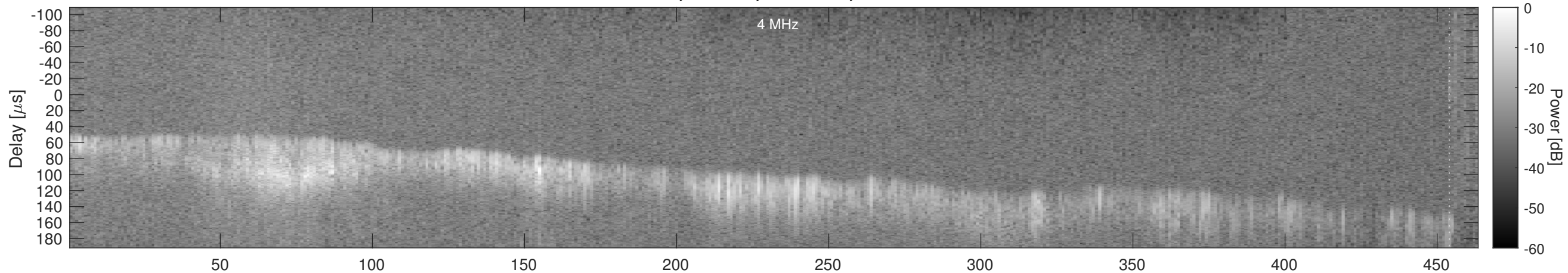
Orbit 16834, Window, Channel 2, Chapman
