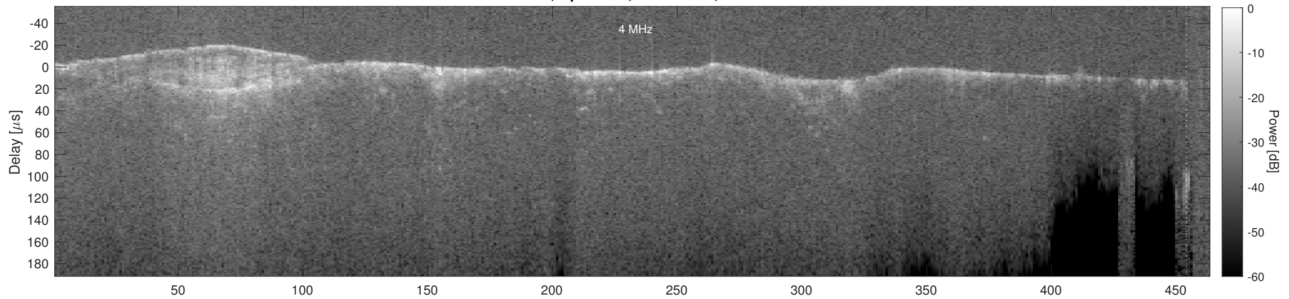
Orbit 16834, Cluttergram
