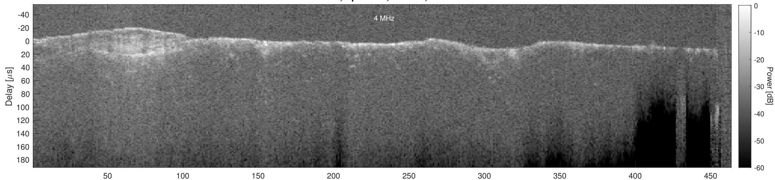
Orbit 16834, Cluttergram
