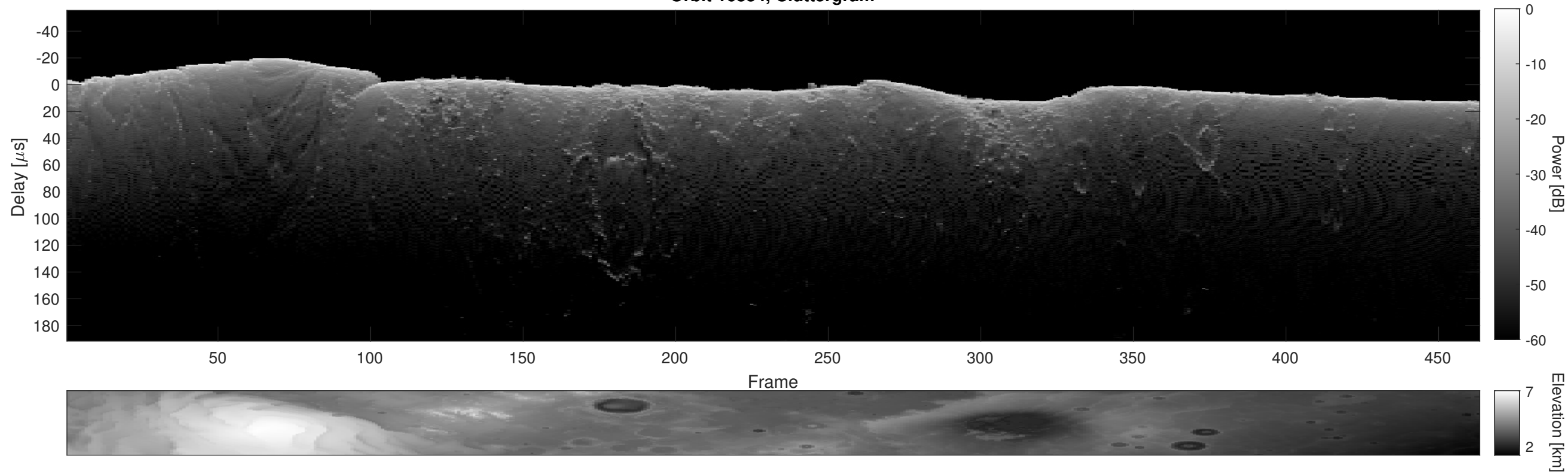
Orbit 16834, Cluttergram
